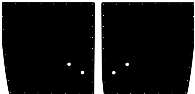
Later 1935-36 Ford Truck (no Garnish) with Upper Upholstery Buttons Leather Grain
